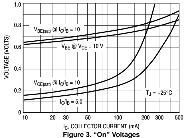
Figure 3. "On" Voltages
